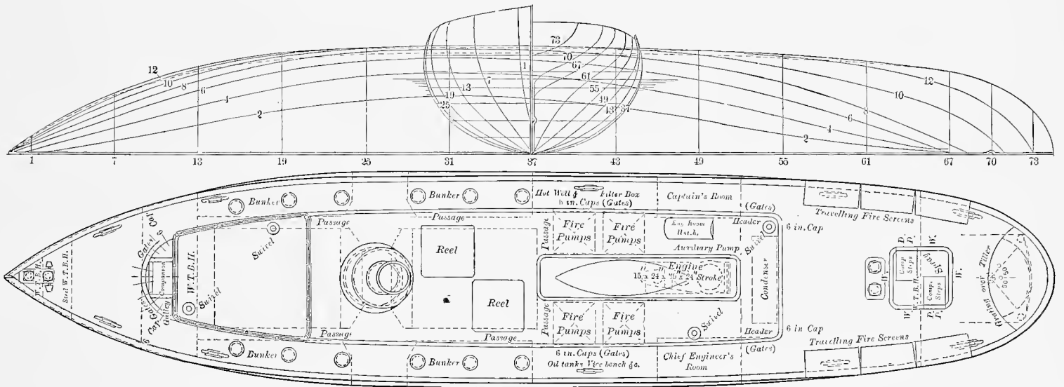
GENERAL PLAN OF THE FIRE BOAT NEW YORKER.
